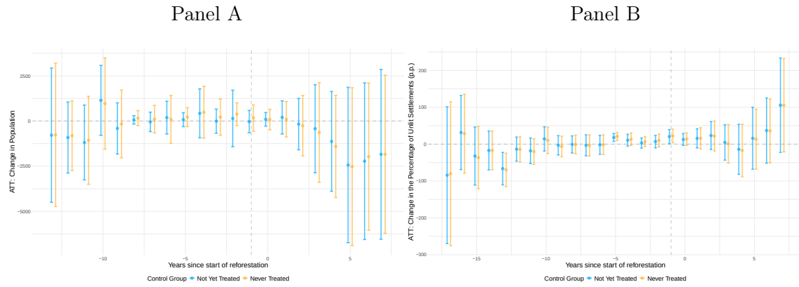
Figure A.21: Impact of NGP on Population
